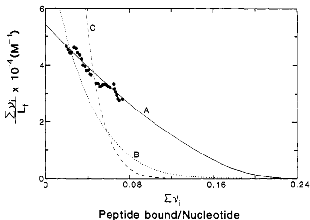
FIGURE 13: The experimental model-independent equilibrium binding isotherm (●) for KWK 2 -NH 2 ( z = +4 ) binding to poly(U) (25.0 °C, pH 6.0, 37 mM Na + ) plotted according to Scatchard (1949) compared with three theoretical models. The continuous curve (A) represents the best-fit isotherm generated using the noncooperative model of McGhee and von Hippel (1974) (see eq 3 in the text) with K_{obs} = 5.4 \times 10^4 \text{ M}^{-1} and n = 4 . The dotted line (B) represents the two-variable model of Manning (1978) using the following parameters: N = 4 , b = 3.8 \text{ \AA} , and [Na^+] = 37 \text{ mM} . The dashed line (C) represents the model of Friedman and Manning (1984) with the parameters K_{obs} = 4.4 \times 10^5 \text{ M}^{-1} and n = N = 4 .
