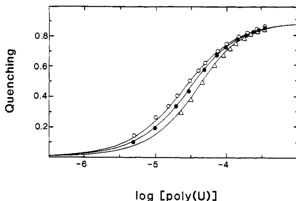
FIGURE 1: Titrations of the oligopeptide, \text{KWK}_2\text{-NH}_2 , with poly(U). Titrations at three peptide concentrations ( 1.8 \mu\text{M} (O), 3.2 \mu\text{M} (●), and 6.0 \mu\text{M} (Δ)) were monitored by the quenching of the peptide tryptophan fluorescence in 37 \text{ mM NaCl} , pH 6.0 (buffer CB), 25.0^\circ\text{C} . The [\text{poly(U)}] is given as moles of nucleotides per liter (M). Solid lines are simulated isotherms generated using eqs 2 and 3, with Q_{\text{max}} = 0.885 , n = 4 nucleotides, and K_{\text{obs}} = 5.4 \times 10^4 \text{ M}^{-1} .
