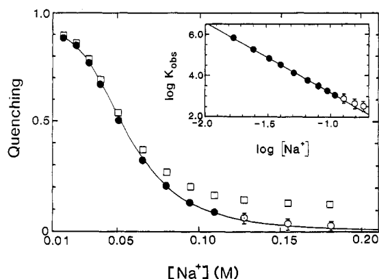
FIGURE 2: Salt-back titration performed by titrating a preformed poly(U)- \text{KWK}_2\text{-NH}_2 complex with \text{NaCl} ( 25.0^\circ\text{C} , pH 6.0) and monitoring the resulting increase in tryptophan fluorescence (decrease in Q_{\text{obs}} ) that accompanies dissociation of the peptide-poly(U) complex. Initial peptide and poly(U) concentrations were 1.48 and 100.5 \mu\text{M} . The squares (□) represent raw data based on observed fluorescence quenching. Circles (O and ●) are the same data after correction for dilution and inner filter effects as described in the text. The inset shows a plot of \log K_{\text{obs}} vs \log [\text{Na}^+] , where the values of K_{\text{obs}} were determined from the salt-back titration using eqs 2 and 3. The linear least-squares line, determined only using the data represented by the closed symbols (●), is \log K_{\text{obs}} = -3.42 \log [\text{Na}^+] - 0.26 . The smooth curve representing the raw data was generated on the basis of eqs 2 and 3.
