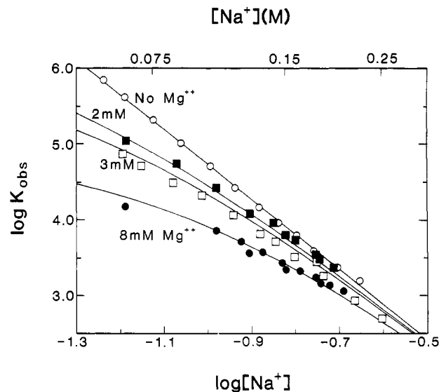
FIGURE 12: The dependence of \log K_{\text{obs}} on \log [\text{Na}^+] (total [\text{Na}^+] ) for the interaction of \text{KWK}_4\text{-NH}_2 ( z = +6 ) with poly(U) in the presence of 0, 2.0, 3.0, and 8.0 mM \text{MgCl}_2 (25.0 °C, buffer CB, pH 6.0). The solid lines are simulated curves based on eqs 13 and 15 and \log K(1 \text{ M}) = 0.28 , z = 6 , \psi = 0.768 .
